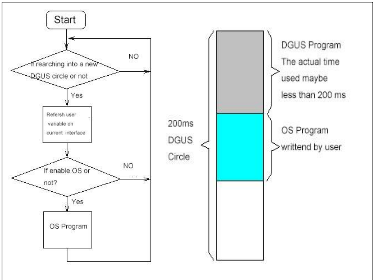
Figure 13 Running Cycle with DWIN OS involved
