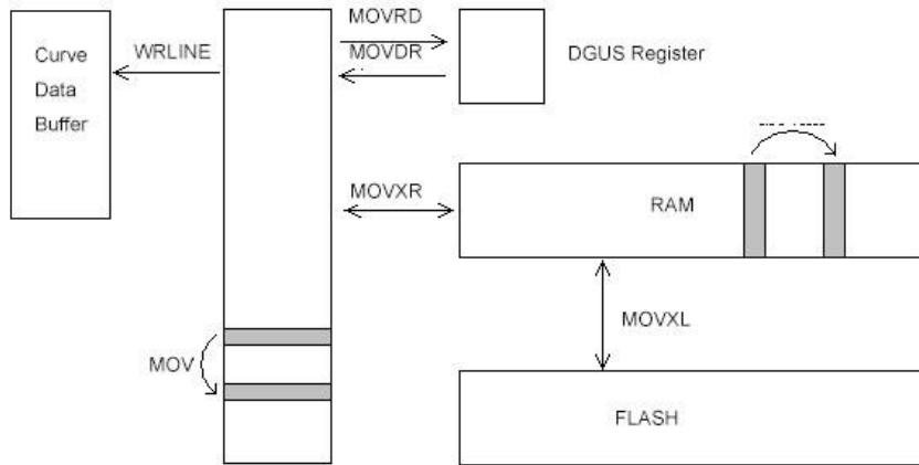
Figure 15 Register that allows OS to addressing
