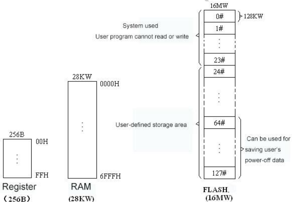
Figure 3 DGUS Register Space
