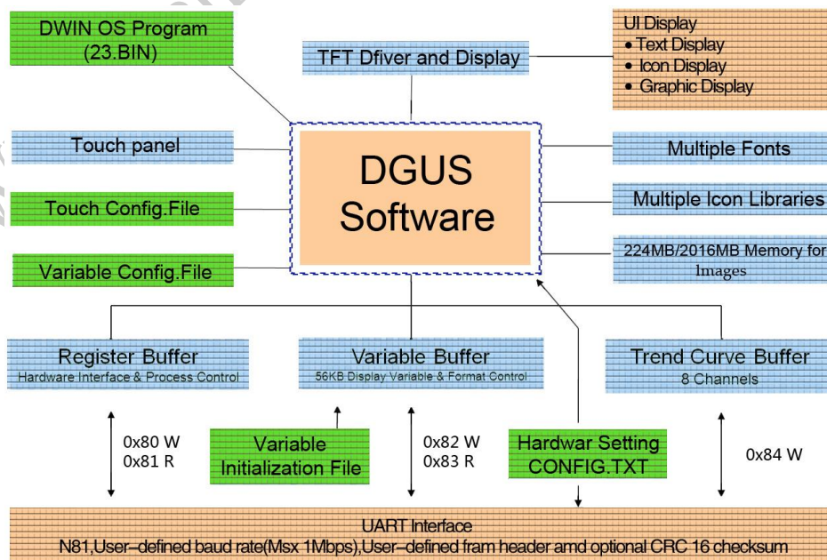
Figure2 Scheme of DGUS software
